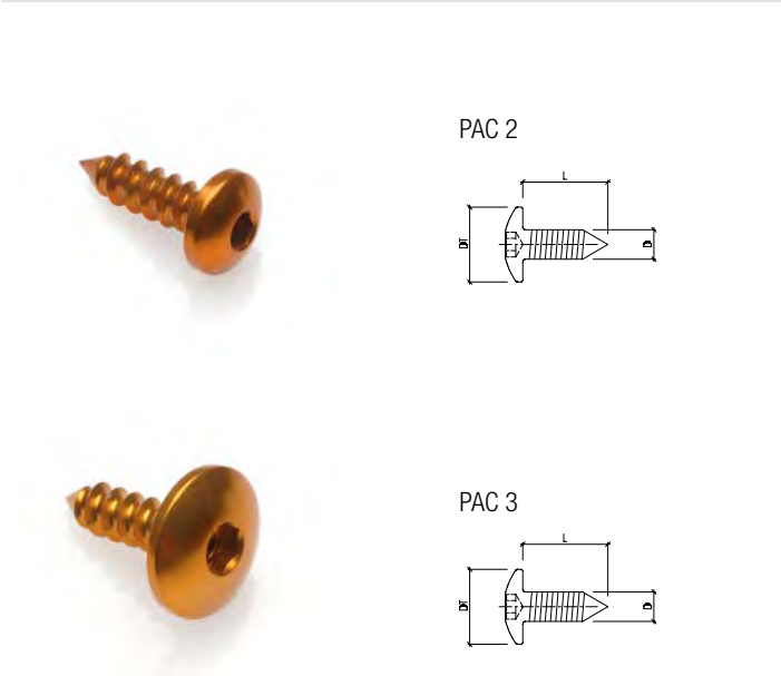
Ergal 7075 / Self tapping bolts - Rosca chapa
